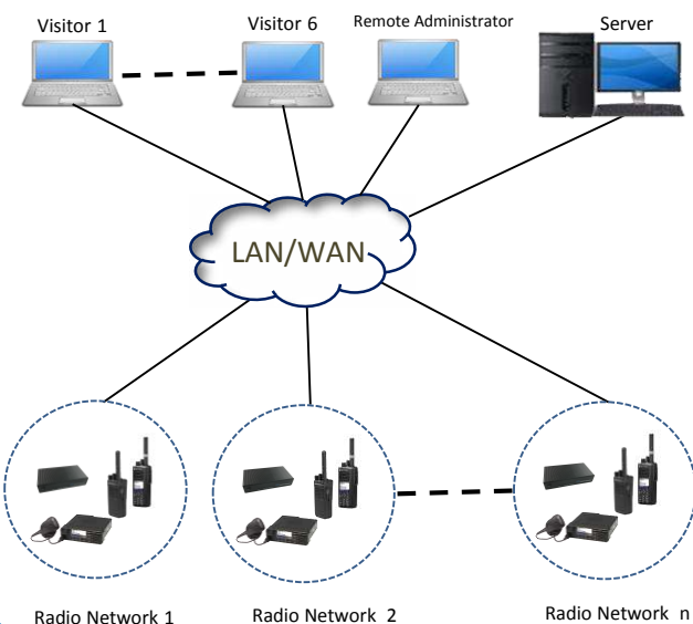
TCE RoIP System Diagram
